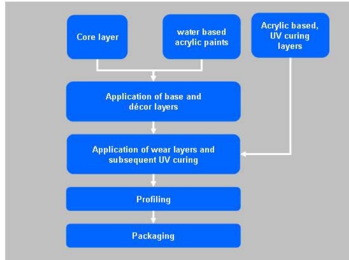
Figure 1: PDL production process
