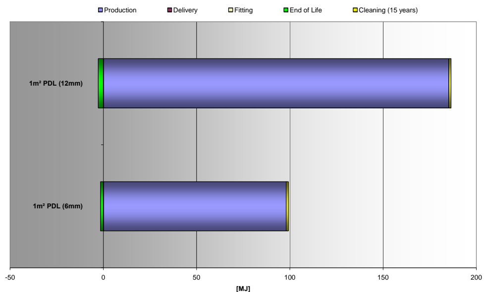
Figure 2: Consumption of renewable primary energy (ref. service life: 15 years)
