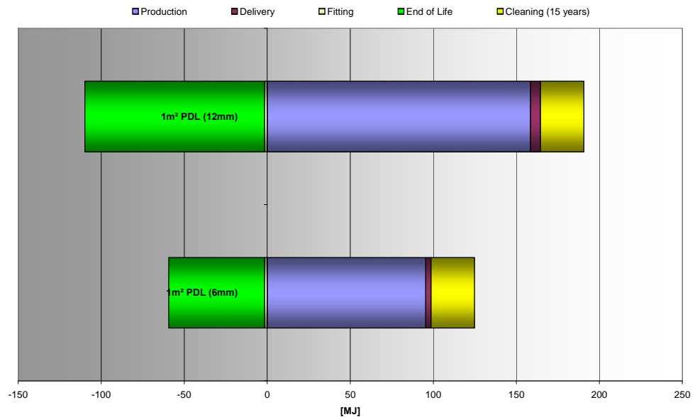
Figure 3: Consumption of non-renewable primary energy for the whole life cycle (reference service life: 15 years)
