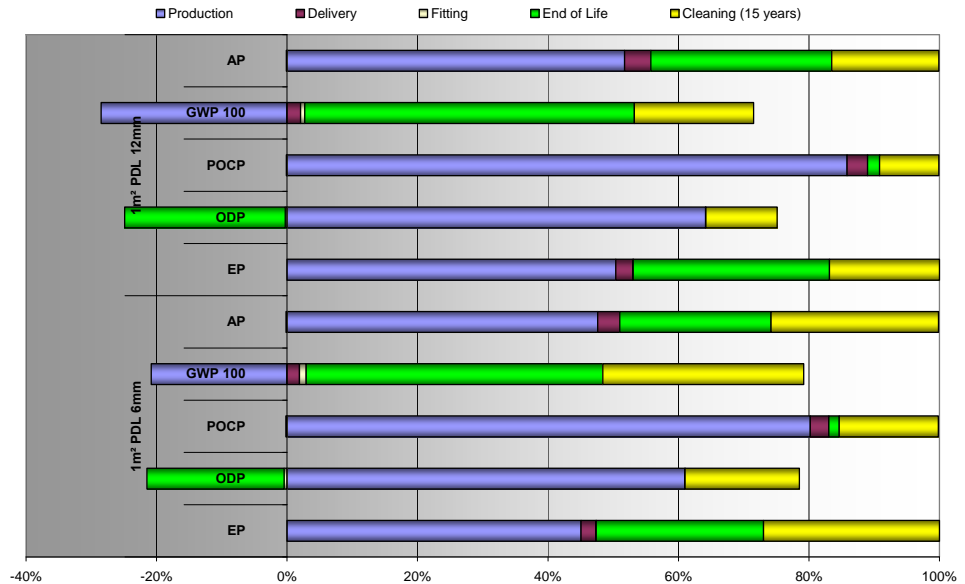
Figure 6: Breakdown of LCA impact categories for all life cycle stages (reference service life: 15 years)
